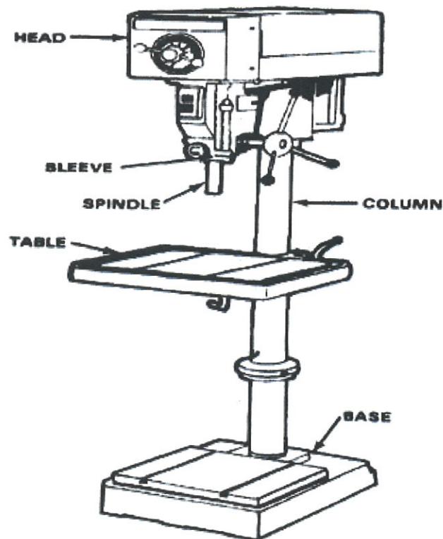
Figure 4-4. Construction of an upright drilling machine
